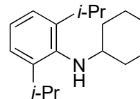
CyanH ( N -cyclohexyl-2,6-diisopropylaniline) (1) 1 H NMR (500 MHz, CDCl 3 )
