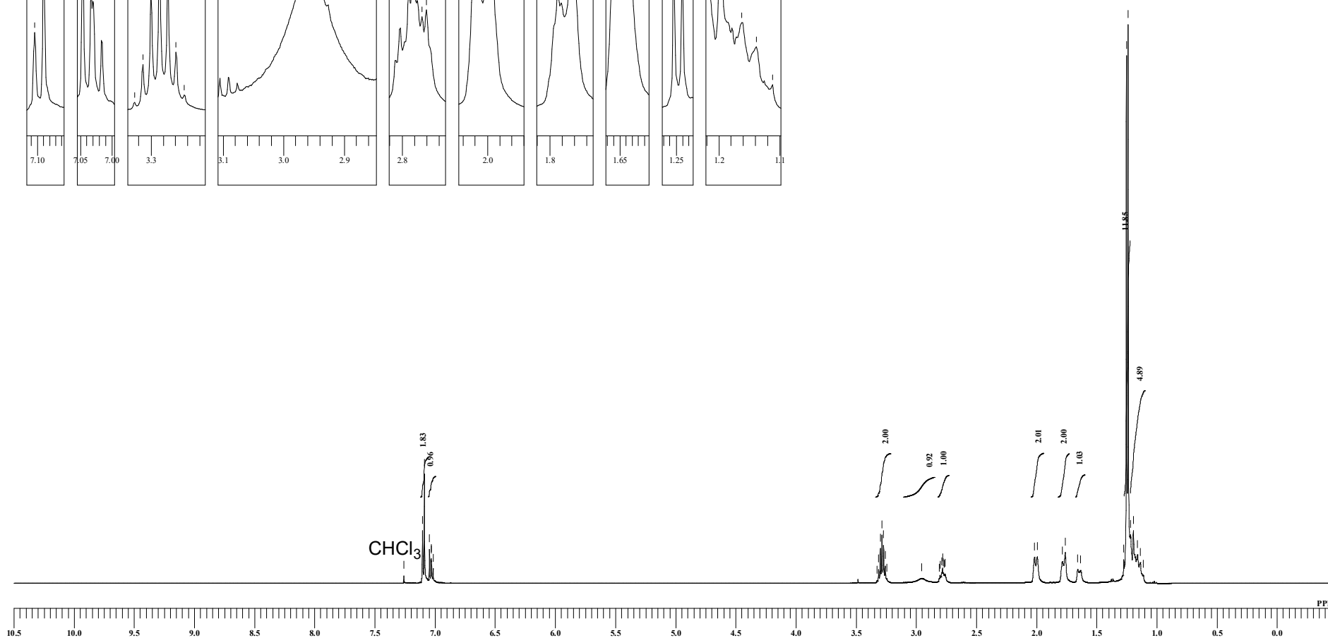
CyanH ( N -cyclohexyl-2,6-diisopropylaniline) (1) 1 H NMR (500 MHz, CDCl 3 )
